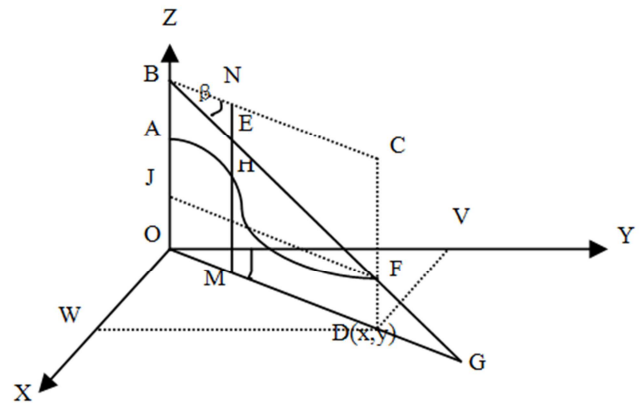
Figure 1. The coordinates of the fire point are calculated according to the rotation angle and pitch angle.
